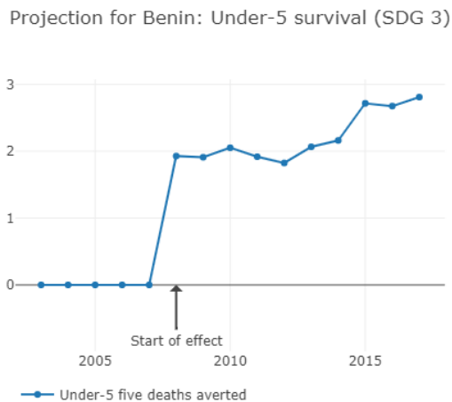
Figure 3 Projection for Benin: Under-5 survival
