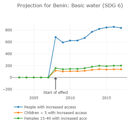
Figure 1 Projection for Benin: Basic drinking water
